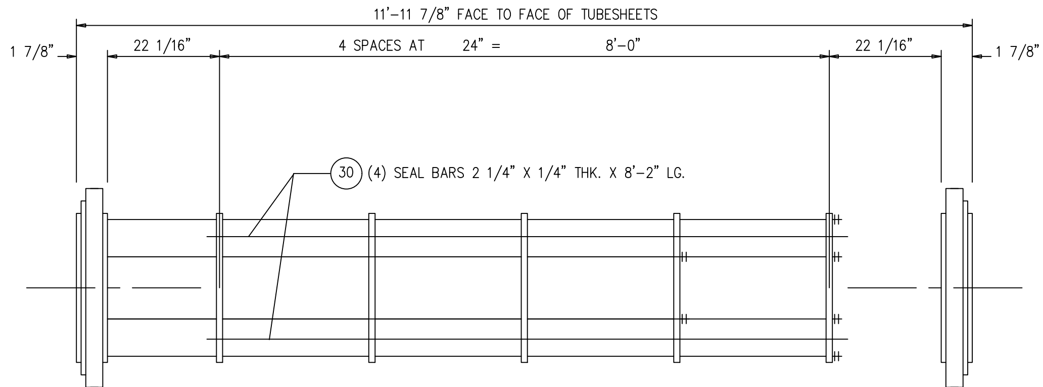
PLAN VIEW
